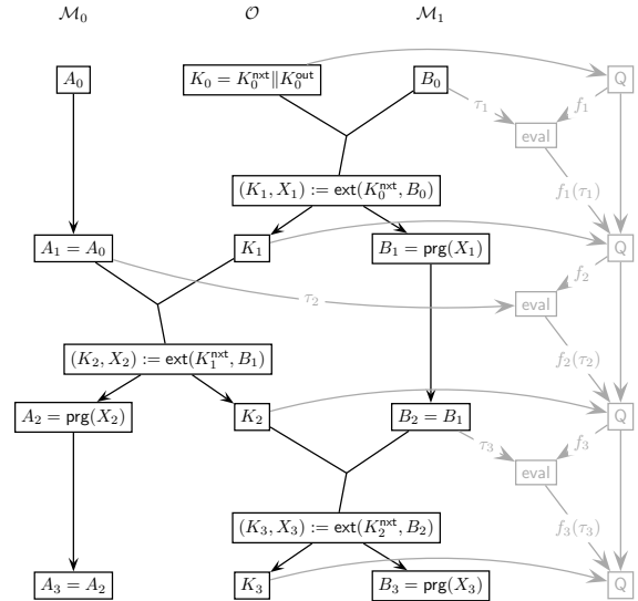
Figure 2. Illustration of the random experiment S(A_0, B_0, K_0) \stackrel{3}{\rightsquigarrow} Q for the stream cipher S as described in Section 2.2.
